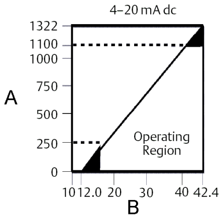
Figure 2: Maximum Load = 40.8 × (Supply Voltage – 12.0)
